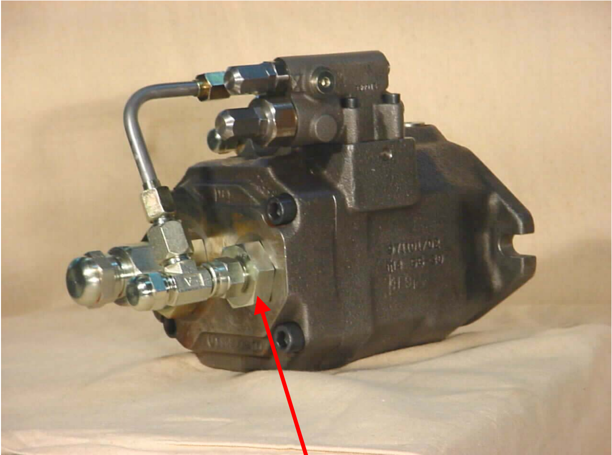
Fitting with orifice
