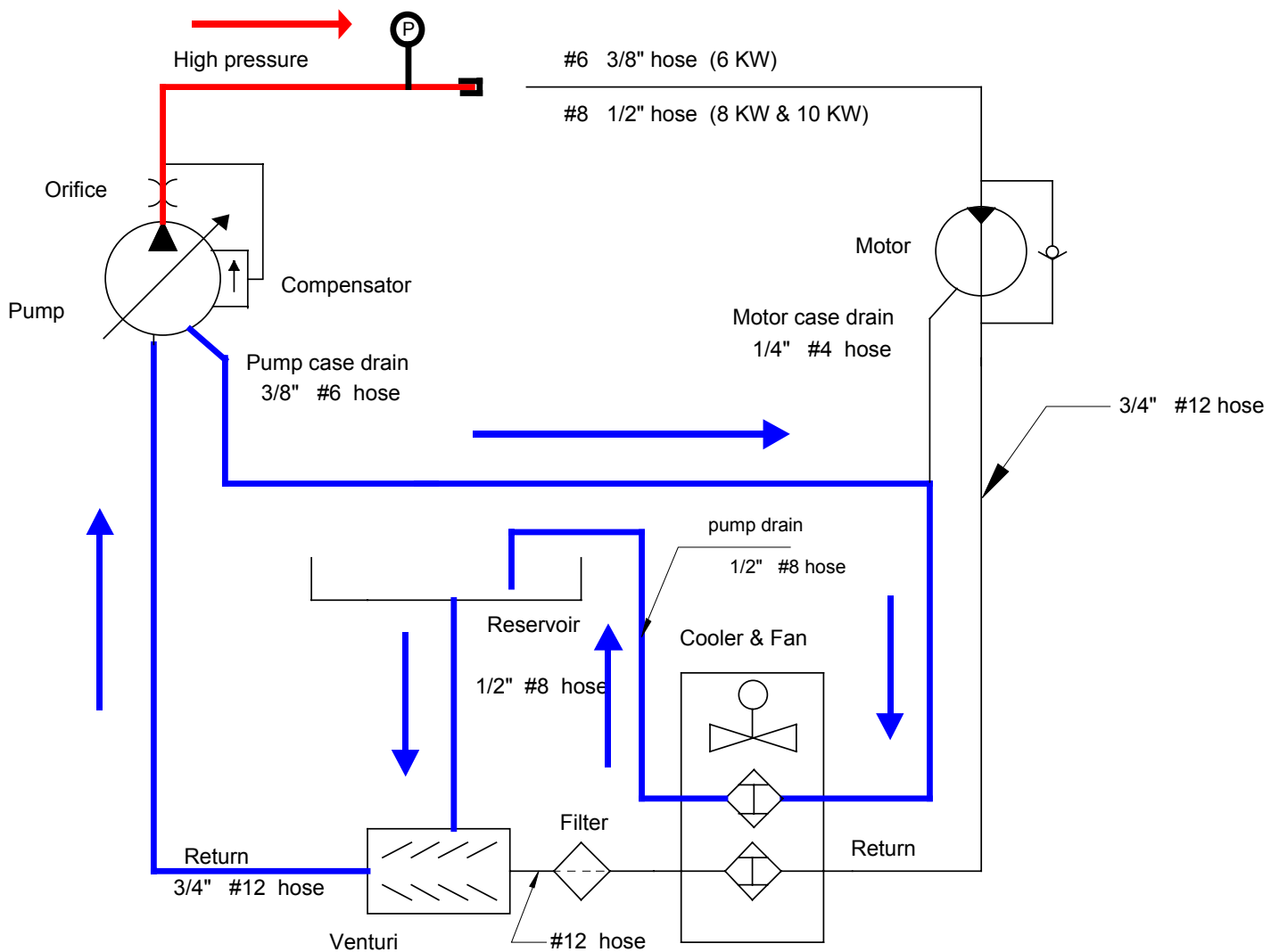
Hart-A-Gen Basic Hydraulic Circuit
